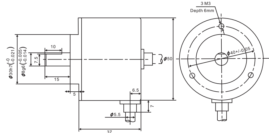
M50SA(Mounting Type A)
